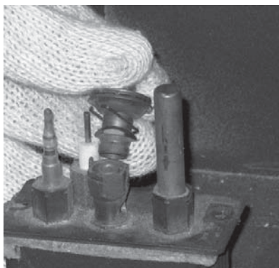
Remove the 2 screws, push Burner Assembly to the left and lift out.
