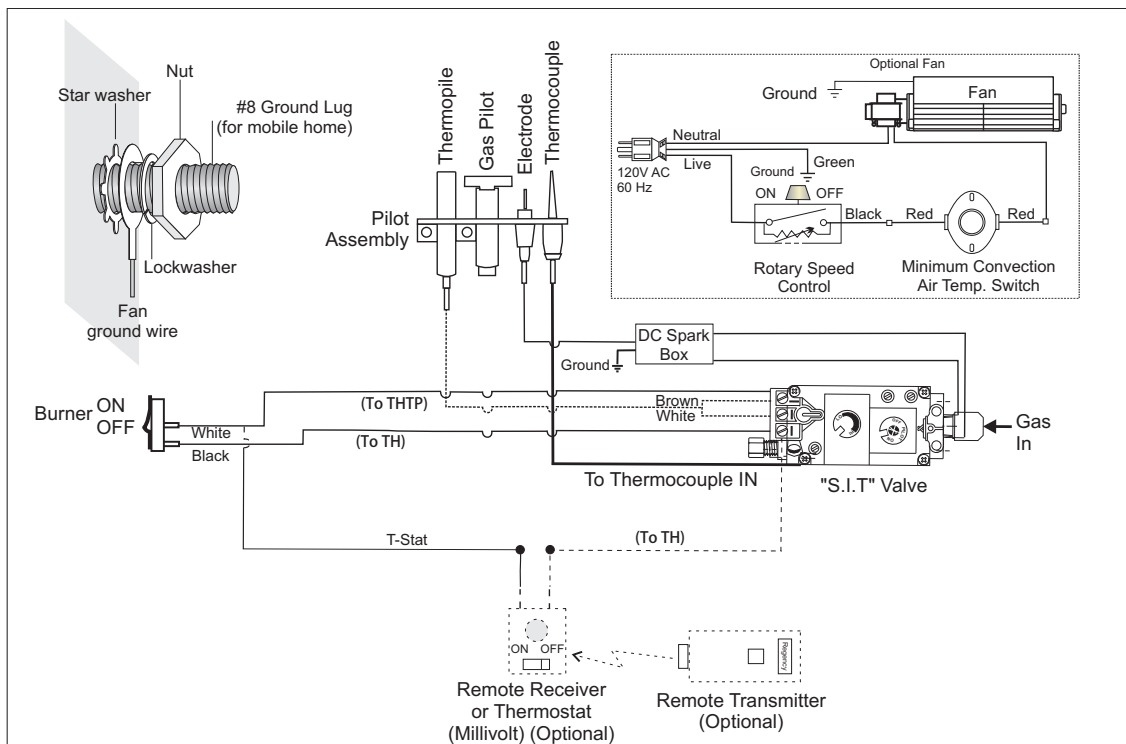
WIRING DIAGRAM FOR GTMF REMOTE
