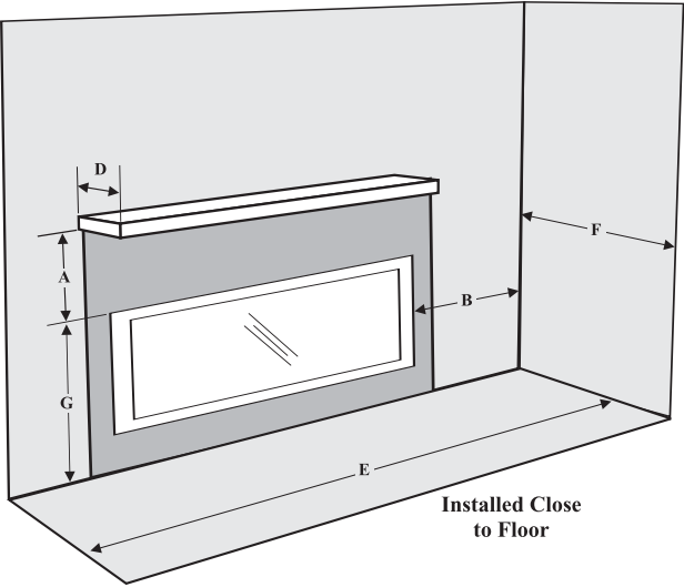
HZ42 Gas Fireplace
